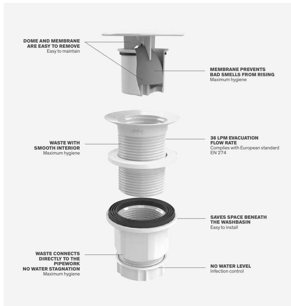
621W cross-section: water-free waste Ref. DELABIE: Coupe3D_621W
